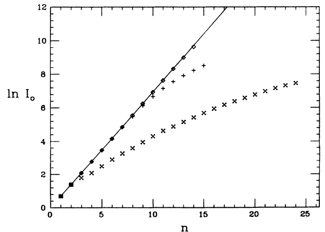
FIG. 2. Quasiperiodic input: \ln I_0(n) as a function of n . I_0(n) is computed from the decimated strings b_{Kn} with K = 1 (cross), K = 4 (plus), and K = 256 (diamond). The full line has the slope equal to the topological entropy of the Bernoulli shift h_{\text{top}} = \ln 2 .
