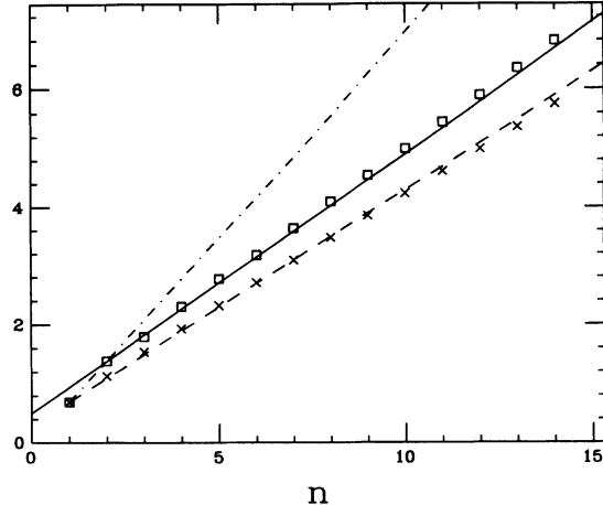
FIG. 6. Random input with \epsilon = 0.5 : \ln I_0(n) (square) and \ln I_1(n) (cross) as a function of n . The slopes of the lines are h_{\text{top}} = 0.44 (full), h_1 = 0.40 (dashed), and K_1 = \ln 2 (dot-dashed).
